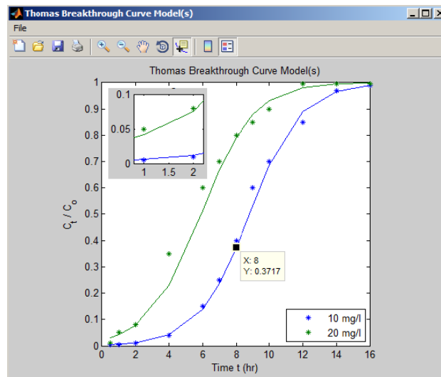
Figure 4. Thomas breakthrough cure models generated by SORPS for concentration 10 mg/l and 20 mg/l, inset plot focusing from 1 to 2 hr and where black spot telling about X-Y coordinates
