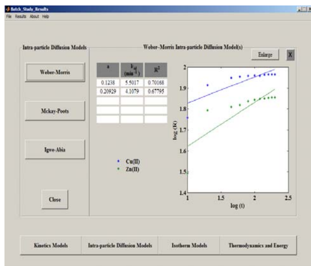
Figure 6. Intra-particle diffusion studies: Weber-Morris
