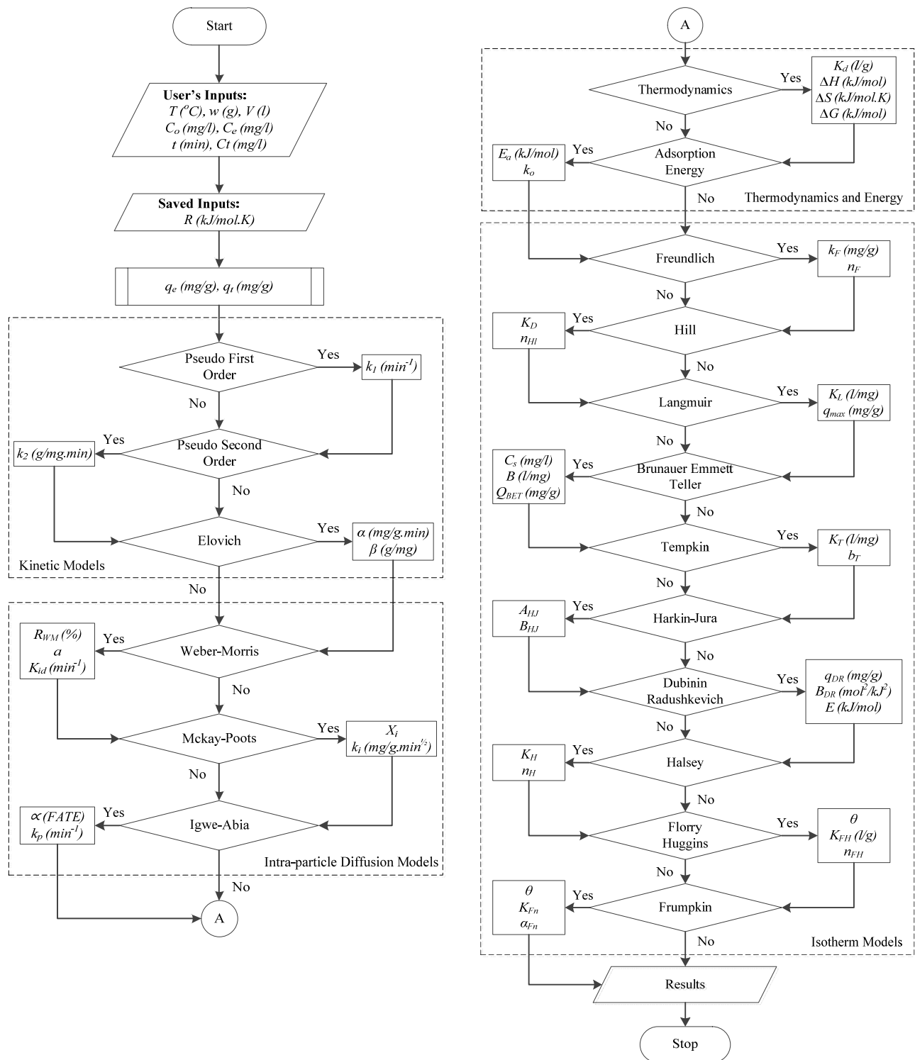
Figure 2. Batch Studies Algorithm
